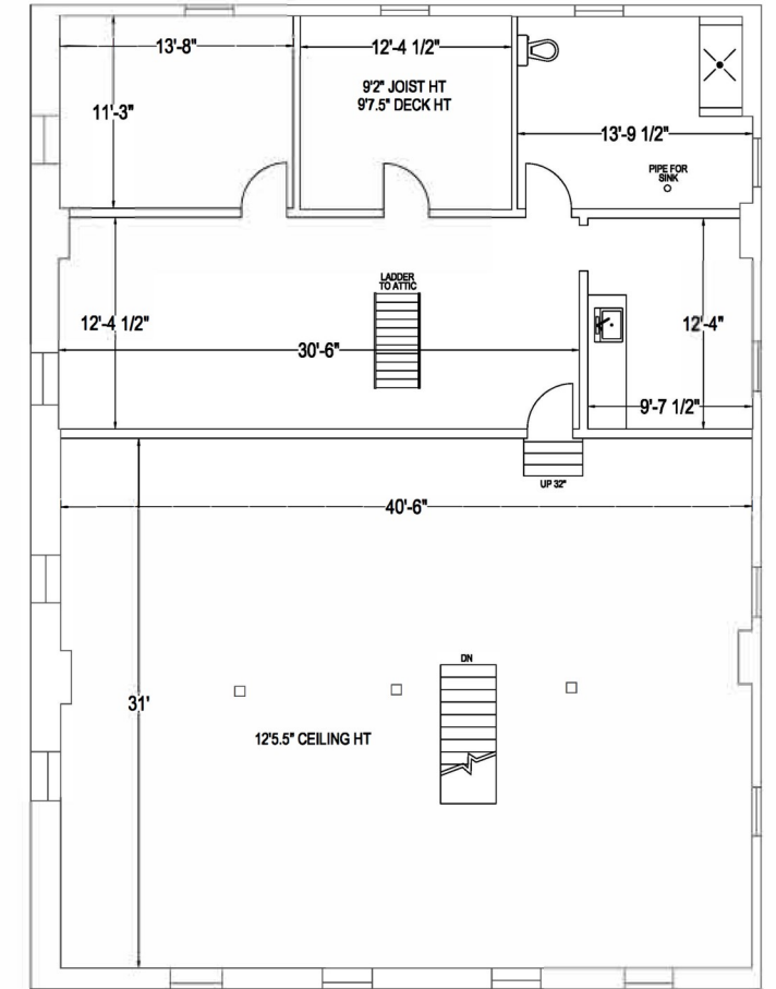
3rd Floor - 2,462Sq ft
