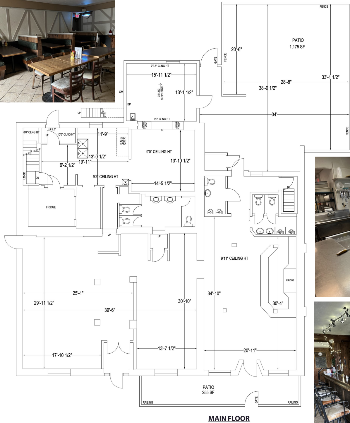
Main Floor - 3,777 Sq ft
